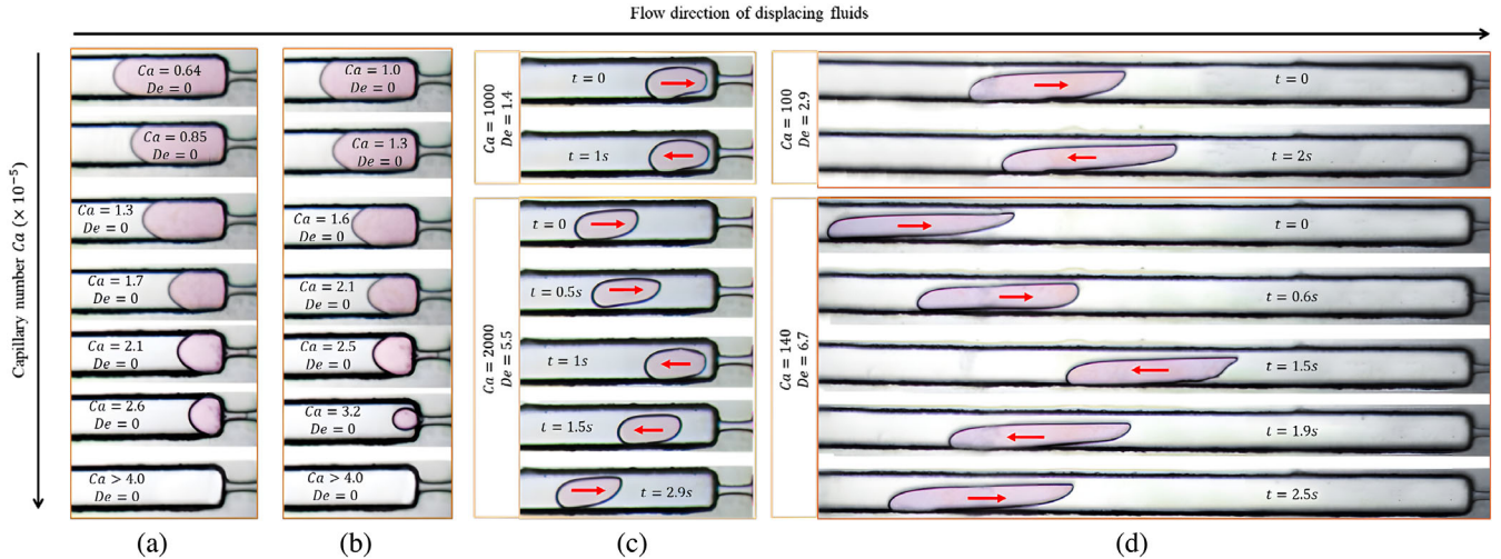
FIG. 1. Viscoelastic fluids induce droplet oscillation. Typical snapshots for the trapped droplets during displacements by (a) Newtonian fluid F_{N1} at flow rates from 1.5 \mu\text{L/h} to 6 \mu\text{L/h} , (b) shear-thinning fluid F_{S1} at flow rates from 0.1 \mu\text{L/h} to 0.35 \mu\text{L/h} , (c) viscoelastic fluid F_{VE4} with a lower relaxation time ( \tau = 0.41 s) at flow rates of 50 \mu\text{L/h} and 200 \mu\text{L/h} , and (d) viscoelastic fluid F_{VE1} with a higher relaxation time ( \tau = 2 s) at flow rates of 70 \mu\text{L/h} and 160 \mu\text{L/h} . The red arrows in (c) and (d) indicate the moving direction of the oscillating droplets.
